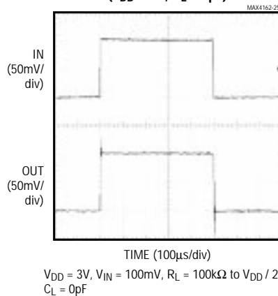
NONINVERTING SMALL-SIGNAL PULSE RESPONSE ( V_{DD} = 3V , C_L = 0\text{pF} )
