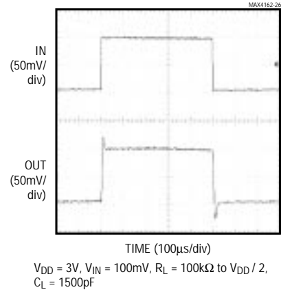
NONINVERTING SMALL-SIGNAL PULSE RESPONSE ( V_{DD} = 3V , C_L = 1500\text{pF} )
