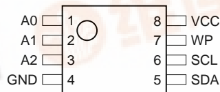
8-Pin SOIC
