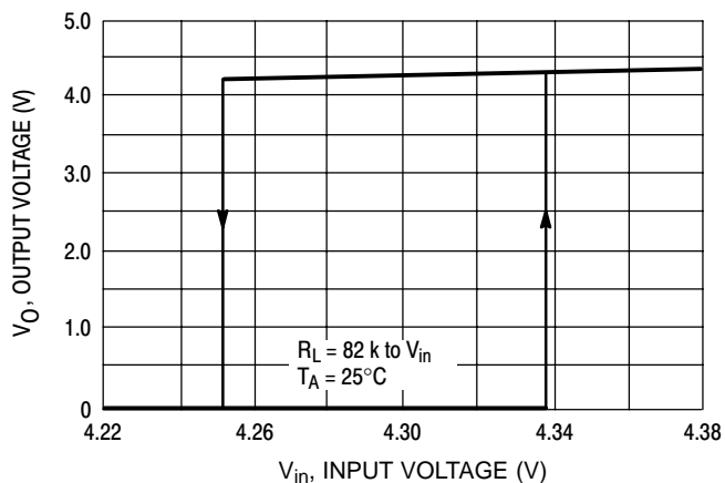
Figure 5. MC3X164-5 Reset Output Voltage versus Input Voltage
