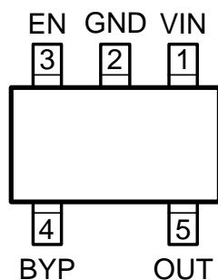
Lead-Free Thin SOT-23-5 (YD5)
