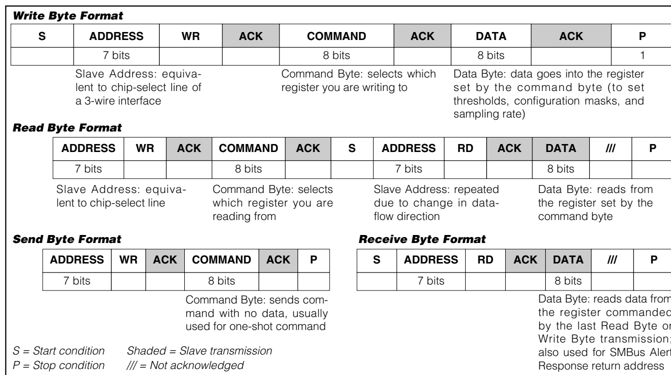
Figure 2. SMBus Protocols
