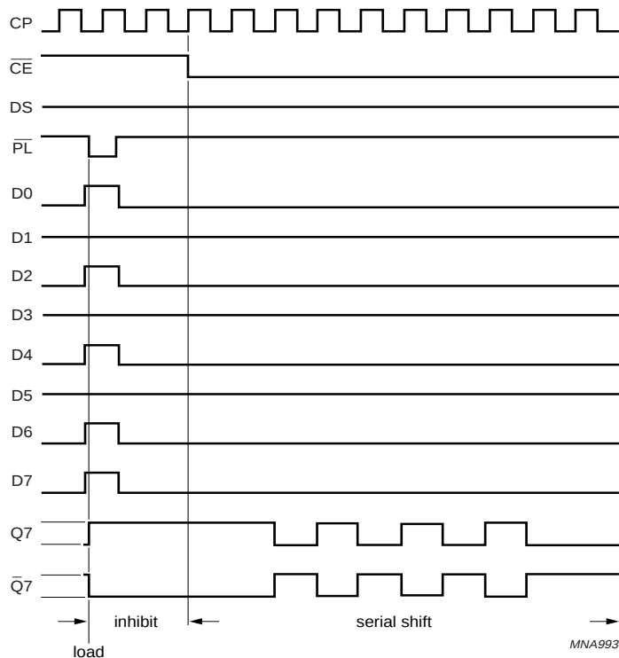
Fig.6 Timing diagram.
