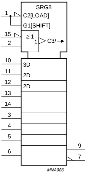
Fig.3 Logic symbol (IEEE/IEC).
