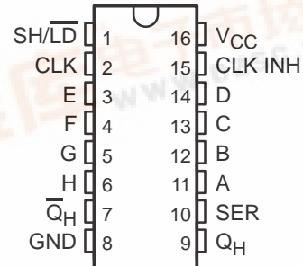
SN54ALS165 ... J PACKAGE SN74ALS165 ... D OR N PACKAGE (TOP VIEW)
