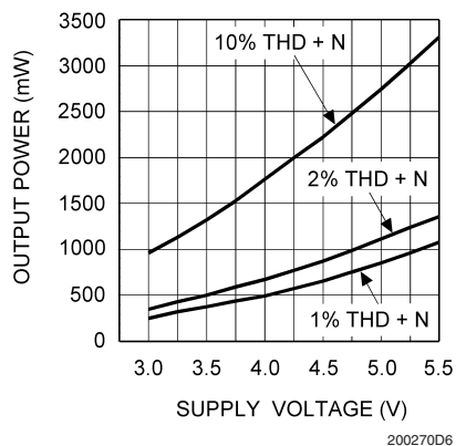
Output Power vs Supply Voltage R_L = 4\Omega + 33\mu\text{H} , f = 1\text{kHz}
