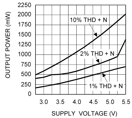
Output Power vs Supply Voltage R_L = 8\Omega + 33\mu\text{H} , f = 1\text{kHz}
