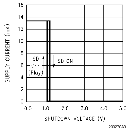
Shutdown Hysteresis Voltage V_{DD} = 5\text{V} , SD Mode = GND (SD High)
