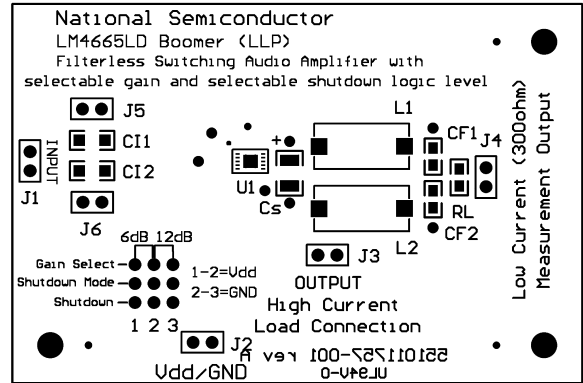
Silk Screen
