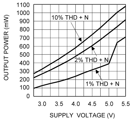
Output Power vs Supply Voltage R_L = 16\Omega + 33\mu\text{H} , f = 1\text{kHz}
