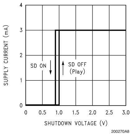
Shutdown Hysteresis Voltage V_{DD} = 3\text{V} , SD Mode = GND (SD Low)
