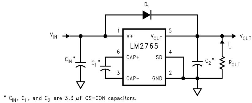
FIGURE 1. LM2765 Test Circuit
