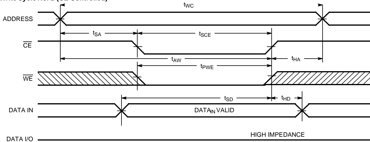
Write Cycle No. 2 ( \overline{CE} Controlled) [8, 12, 13]
