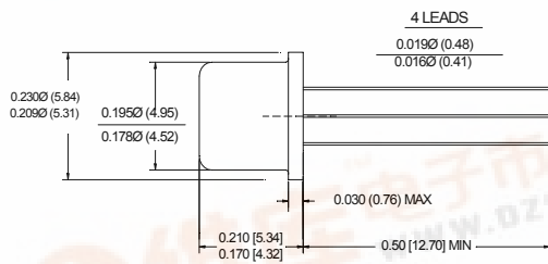
DIMENSIONS ARE IN INCHES (MILLIMETERS)
