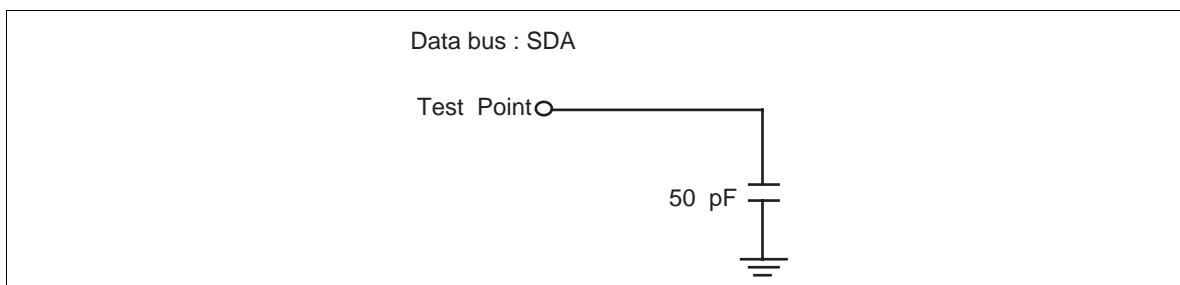
Figure 56 Load Circuit
