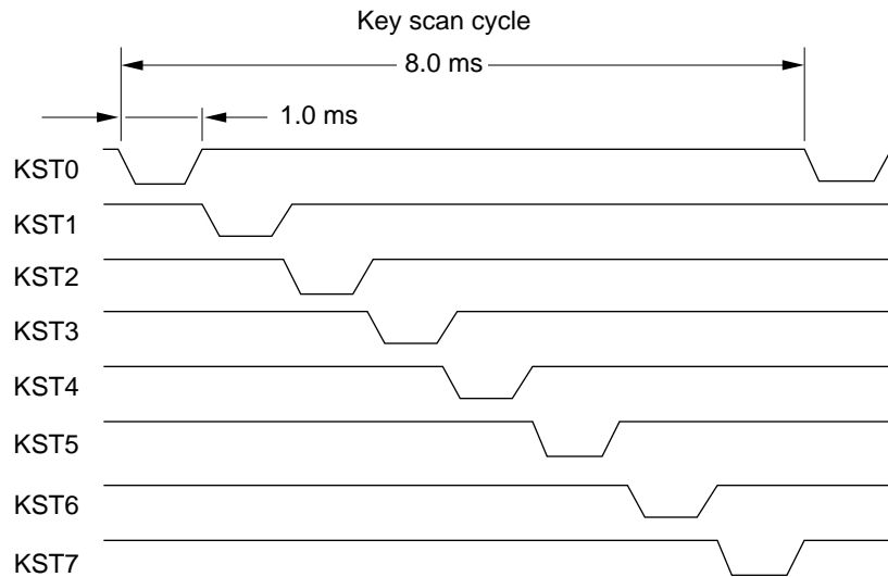
Figure 27 Key Strobe Output Timing (NL1 = 1, KF1/0 = 10, fcp/fosc = 160 kHz)
