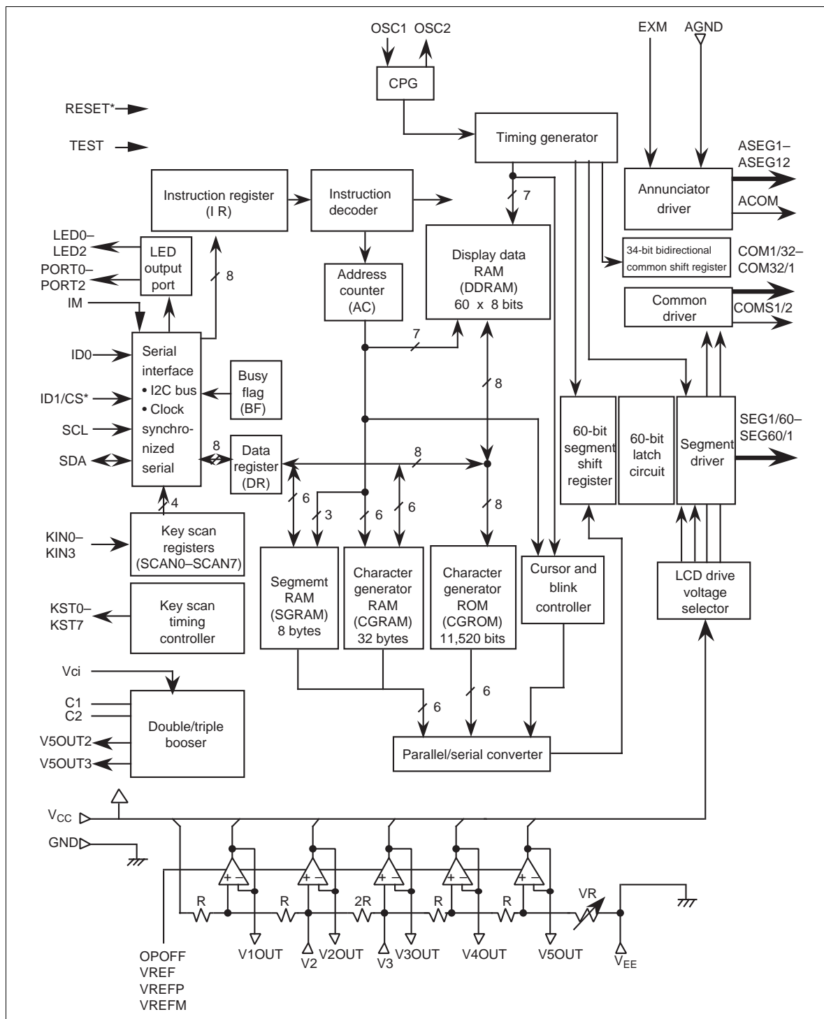
HD66727 Block Diagram
