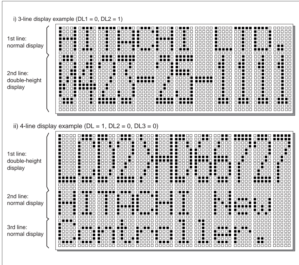
Figure 46 Double-Height Display Examples
