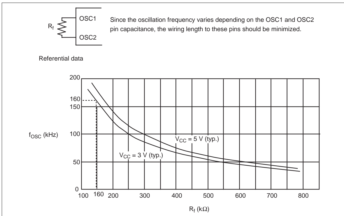
Figure 54 Internal Oscillation
