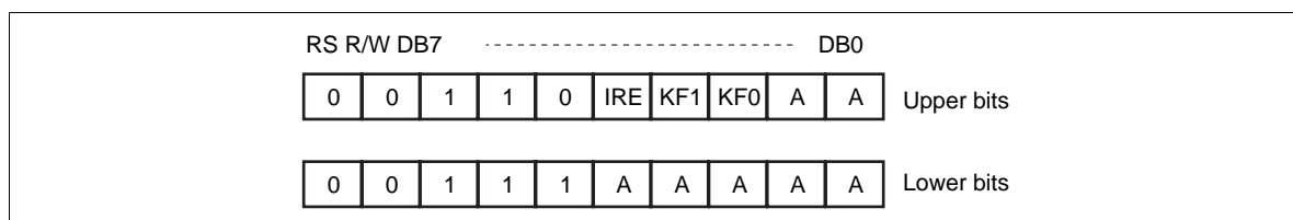
Figure 20 DDRAM Address Set Instruction
