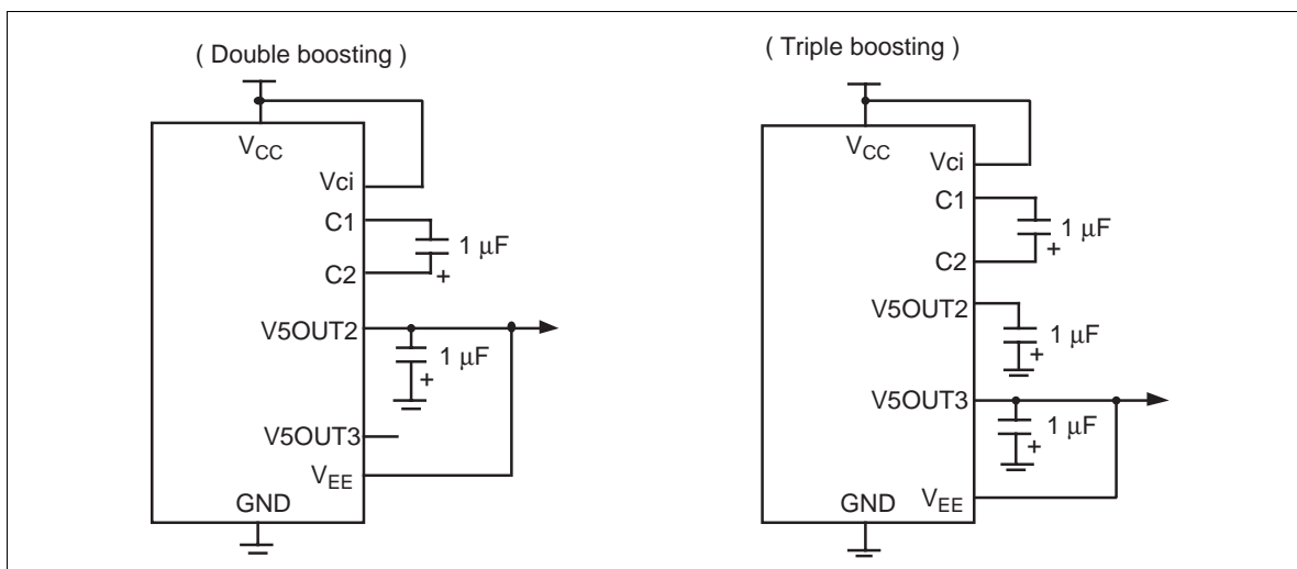
Figure 55 Booster
