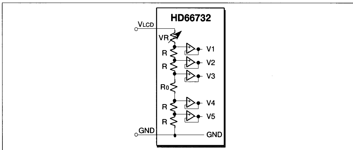
Figure 10 Contrast Adjuster
