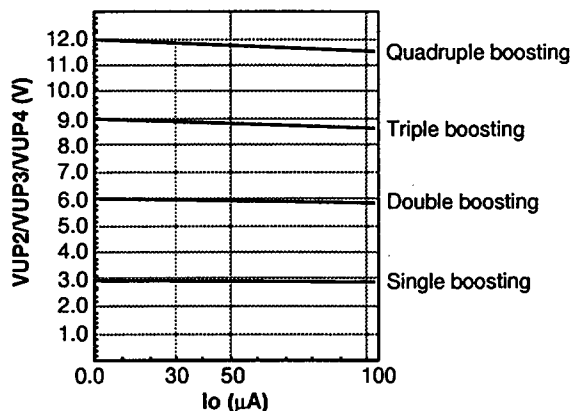
Figure 69 Booster (cont)
