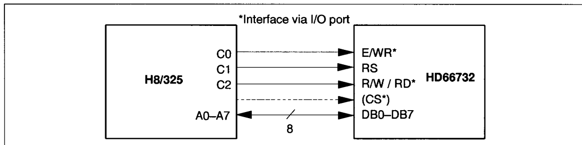
Figure 31 Interface to 8-bit Microcomputer
