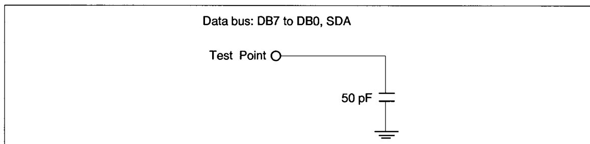
Figure 70 Load Circuit
