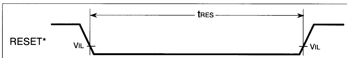
Figure 74 Reset Timing
