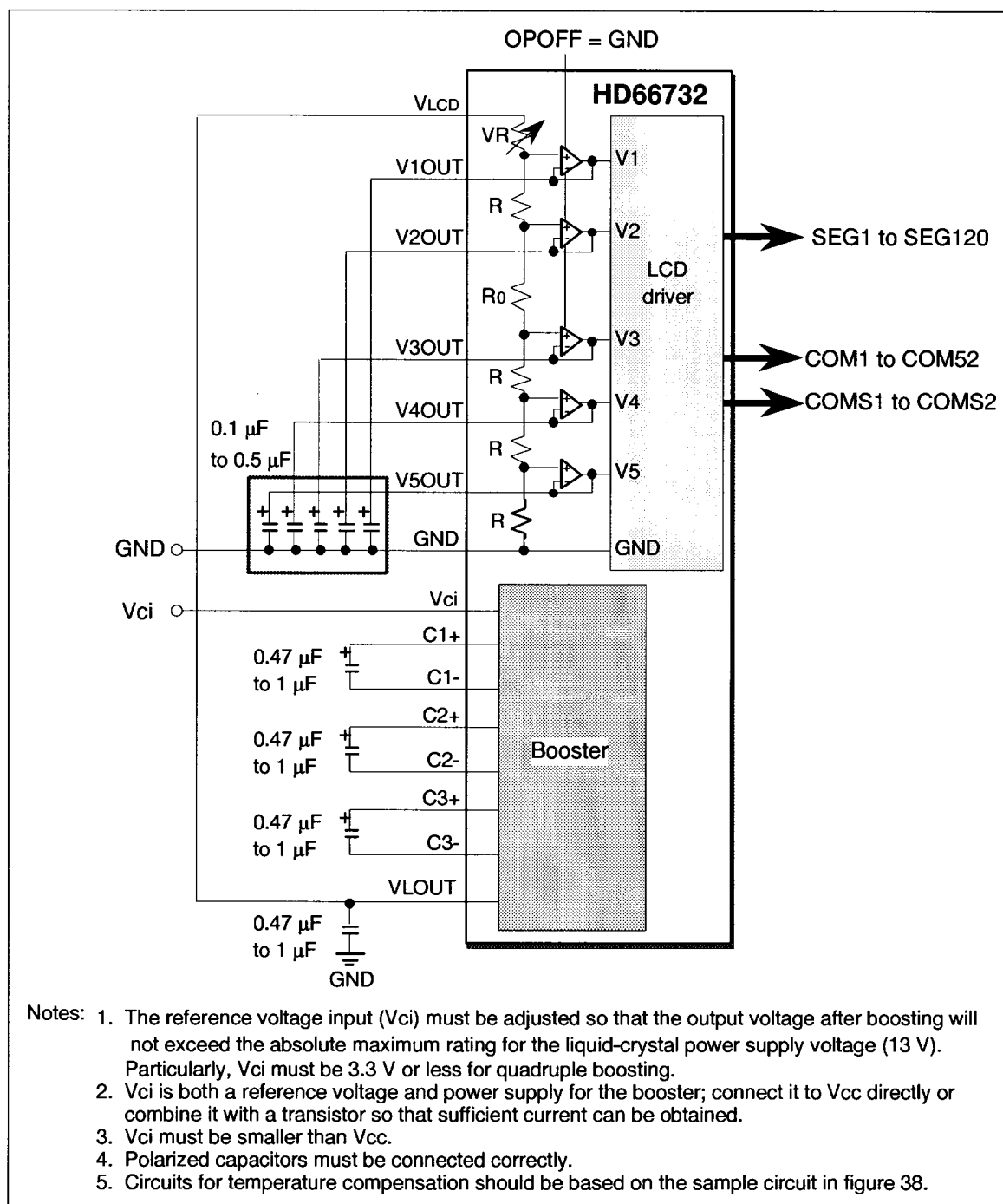
Figure 37 Internal Booster for LCD Drive Voltage Generation
