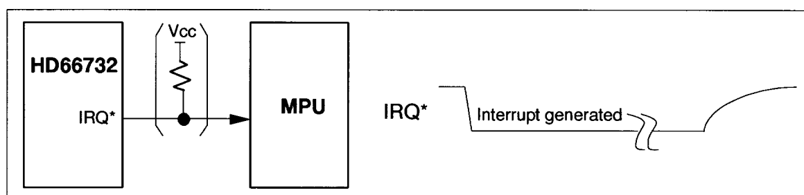
Figure 29 Interrupt Generator
