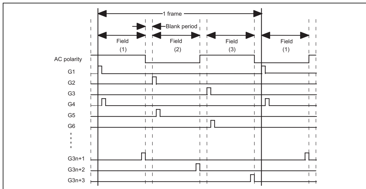
Gate output timing during 3-field interlaced drive
