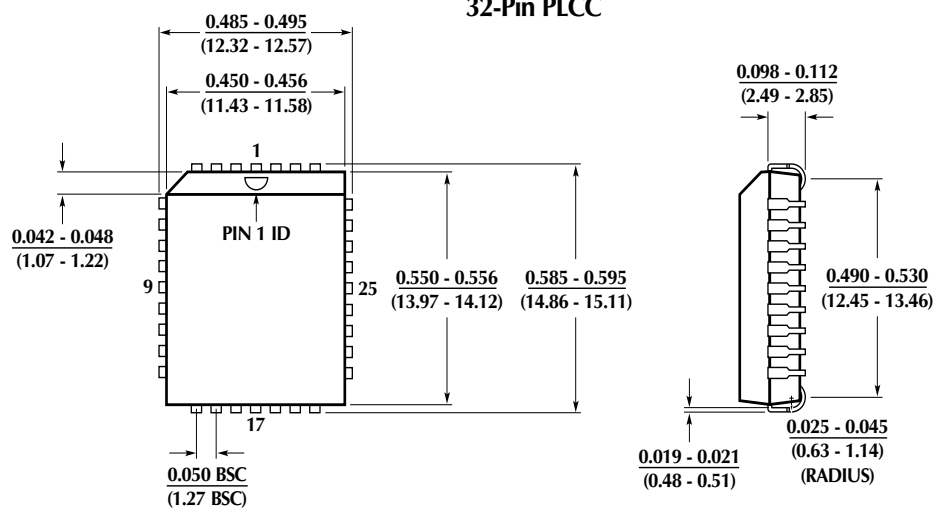
Package: Q32 32-Pin PLCC
