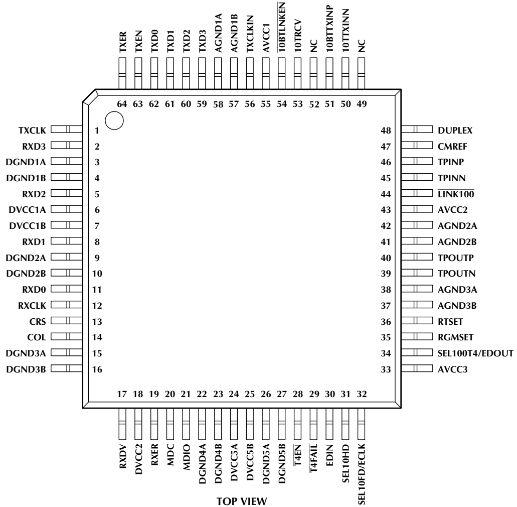
ML6692 64-Pin TQFP (H64-10)
