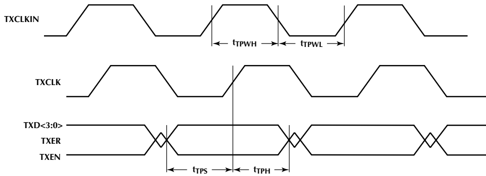
Figure 2. MII Transmit Timing
