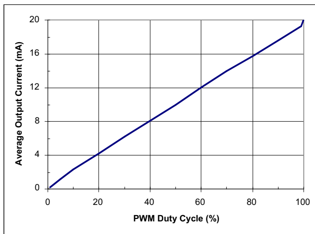
Fig. 2 Average I_o vs SHDN duty cycle
