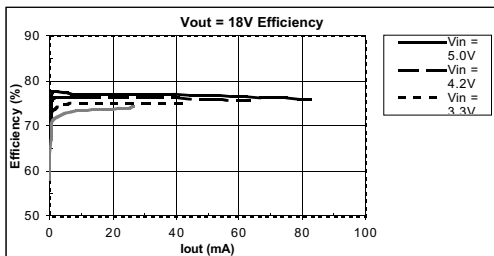
Figure 5. 18V Output Efficiency
