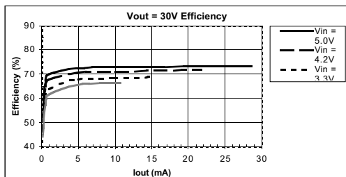
Figure 11. 30V Output Efficiency
