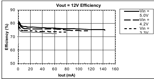
Figure 1. 12V Output Efficiency
