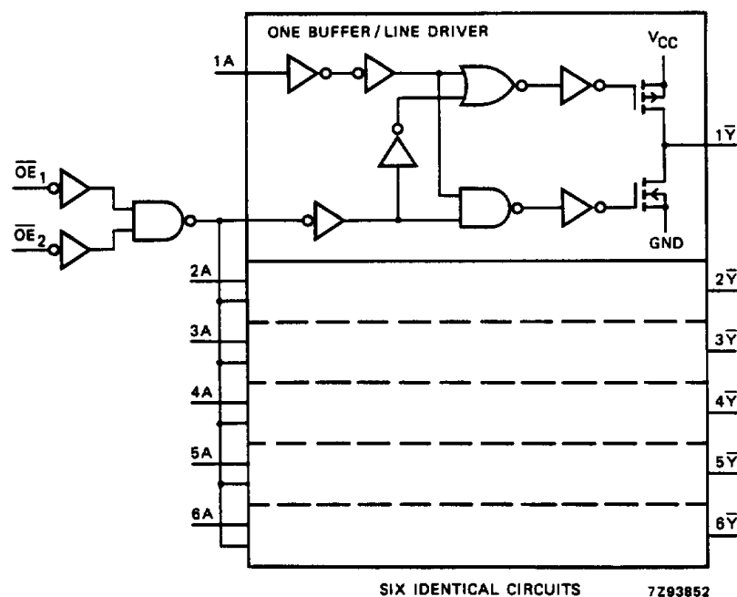
Fig.5 Logic diagram.
