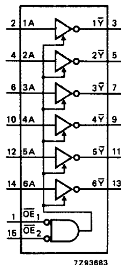
Fig.4 Functional diagram.
