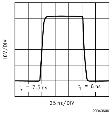
FIGURE 5. LM2466 Pulse Response
