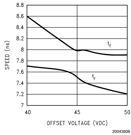
FIGURE 7. Speed vs Offset
