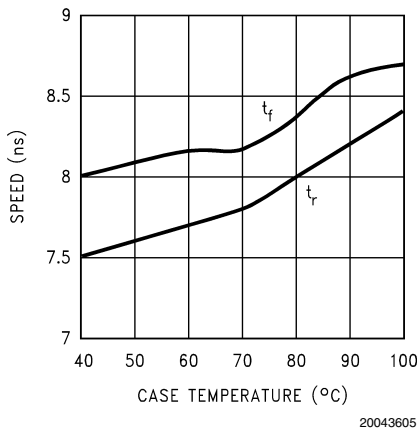
FIGURE 4. Speed vs Temp.
