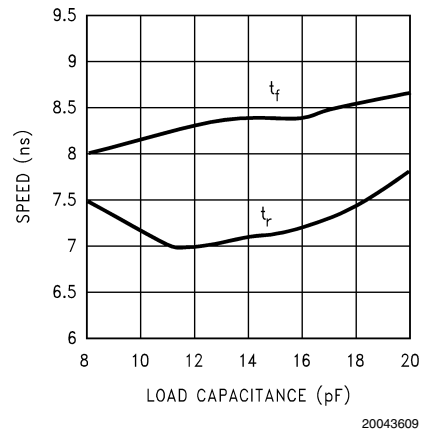
Speed vs Load Capacitance
