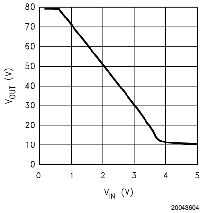
FIGURE 3. V_{OUT} vs V_{IN}
