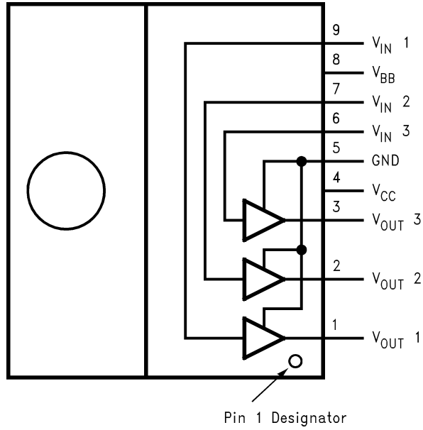
Top View Order Number LM2466TA
