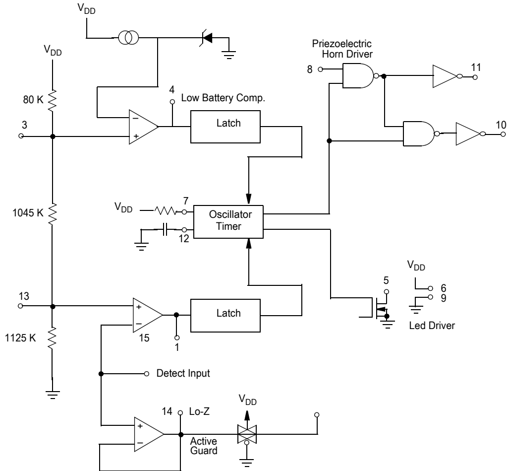
Figure 2. Block Diagram
