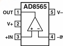
5-Lead SC70 (KS Suffix)
