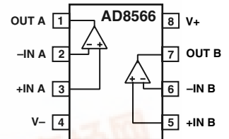
8-Lead MSOP (RM Suffix)
