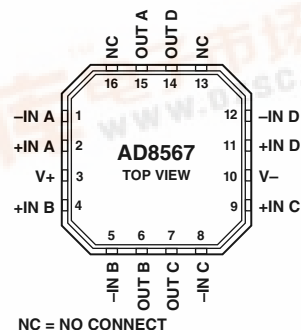
16-Lead CSP (CP Suffix)
