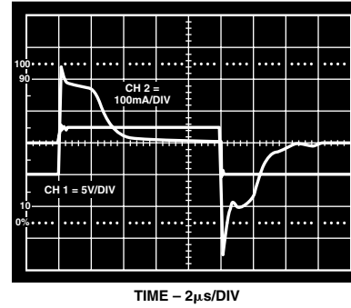
Figure 6. Scope Photo of the V_{COM} Instantaneous Peak Current
