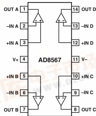
14-Lead TSSOP (RU Suffix)
