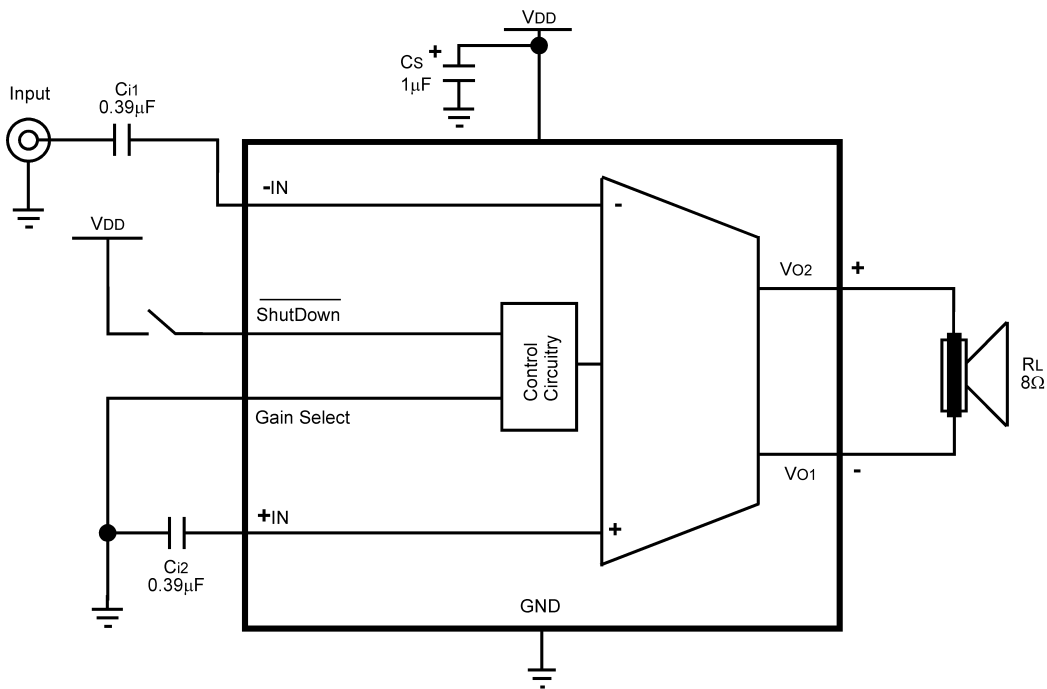
FIGURE 3. Single-Ended Input with high gain selection configuration
