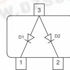
BAT68-06 BAT68-06W
