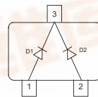
BAT68-05 BAT68-05W
