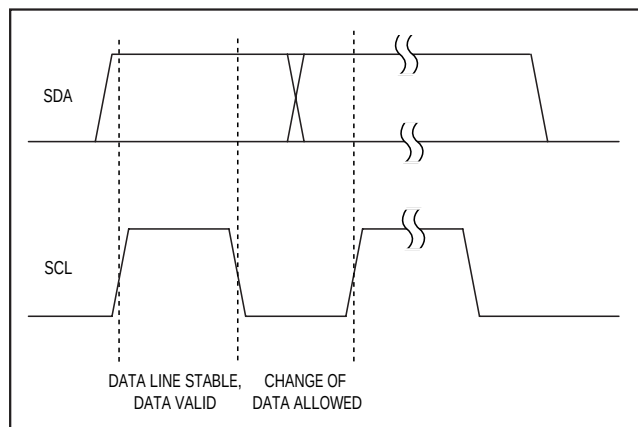
Figure 3. Bit Transfer
