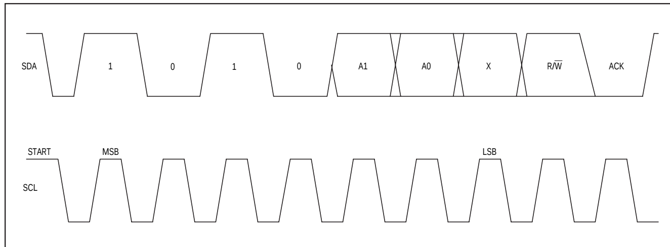
Figure 6. Slave Address
