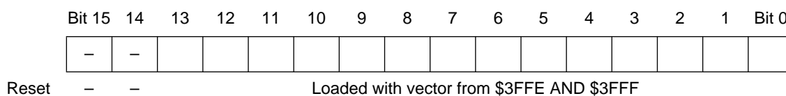
Figure 3-5. Program Counter
