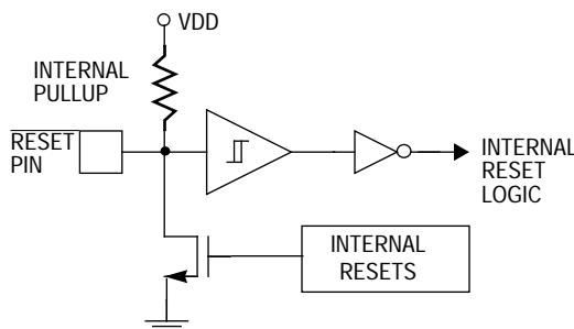
Figure 5-1. Internal Resets
