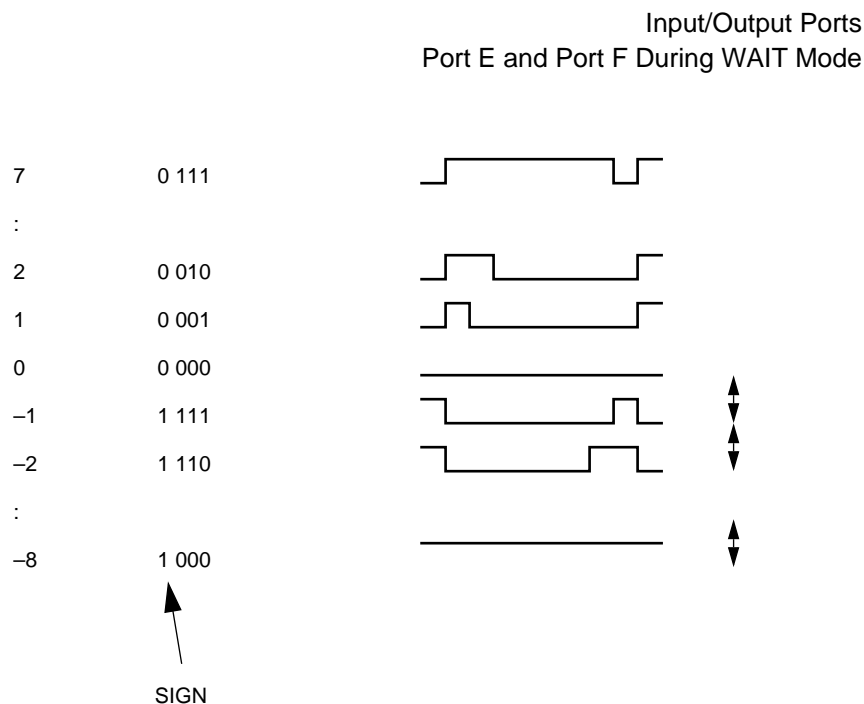
Figure 7-16. Correspondence between Data and PWM Values
