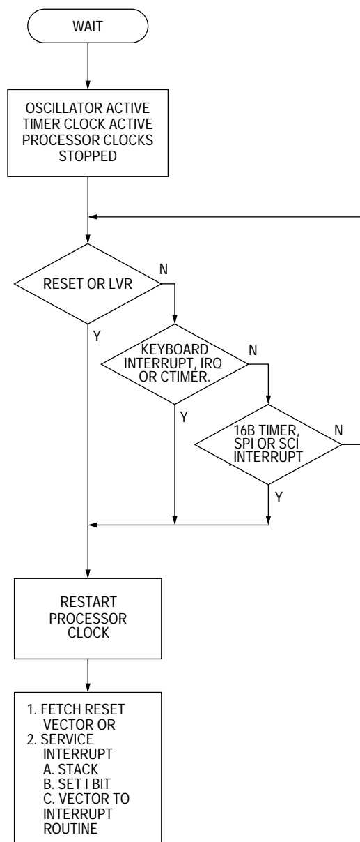
Figure 6-1. WAIT Flowchart
