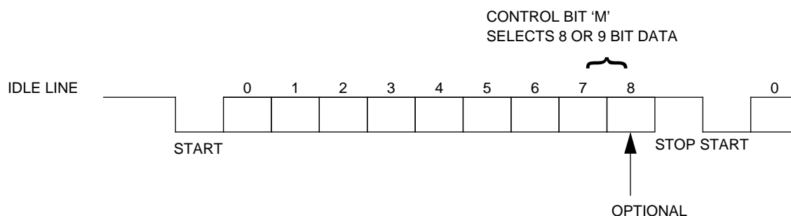
Figure 11-2. Data Format
