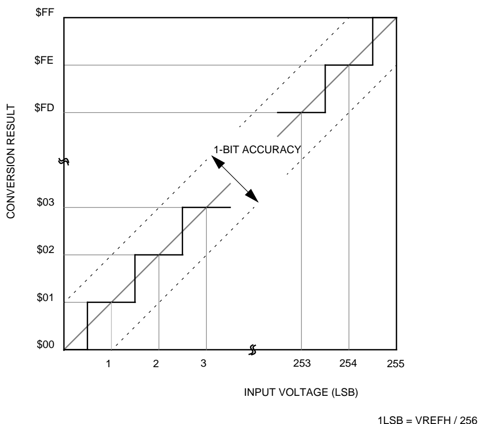
Figure 12-4. Transfer Curve of an Ideal 8-Bit A/D Converter
