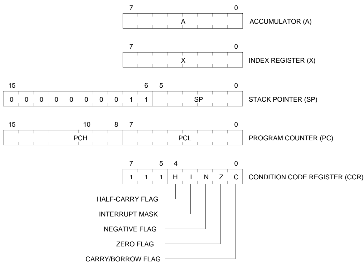
Figure 3-1. Programming Model
