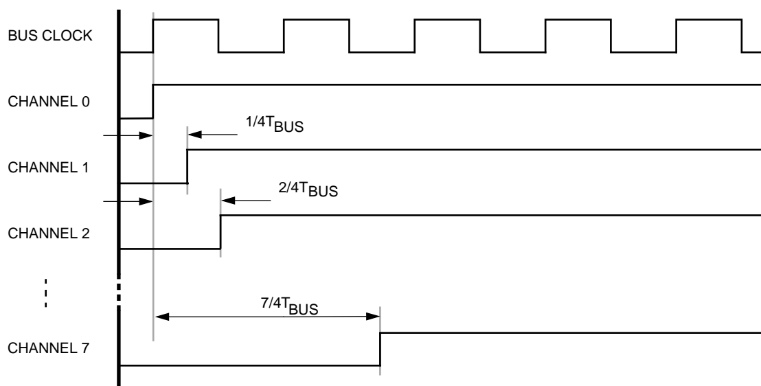
Figure 14-2. PWM Microshifts
