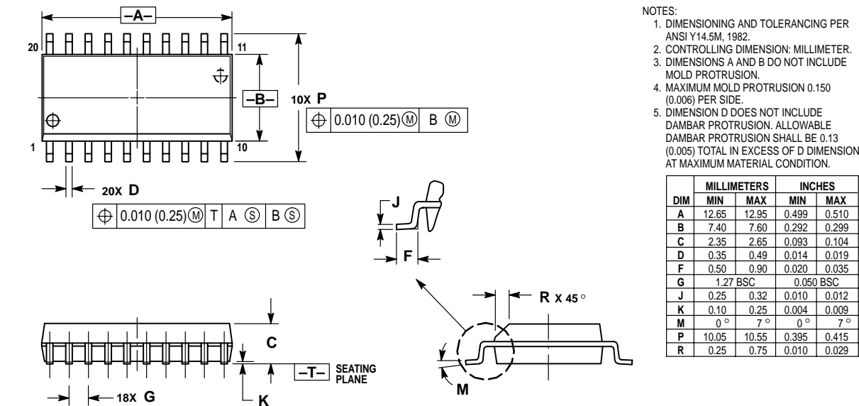
Figure 14-3. 20-Pin SOIC Mechanical Dimensions
