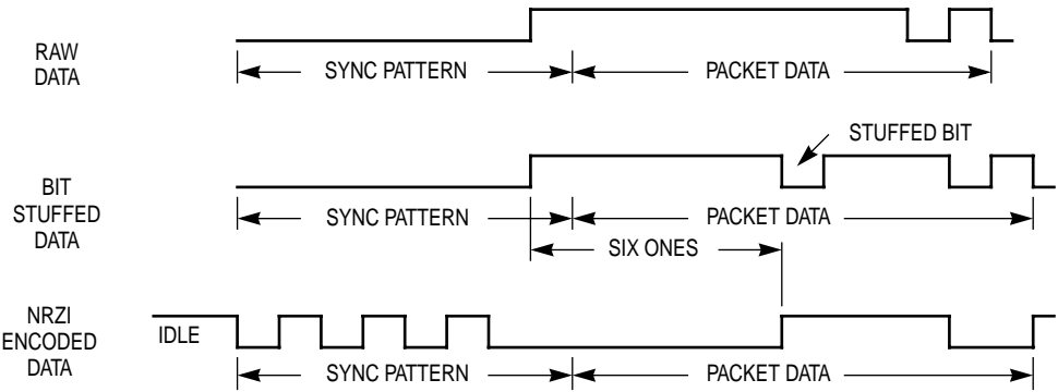
Figure 10-18. Bit Stuffing
