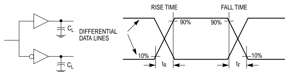
Figure 10-15. Data Signal Rise and Fall Time
