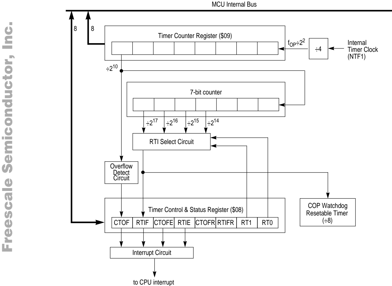
Figure 8-1. Multi-Function Timer Block Diagram
