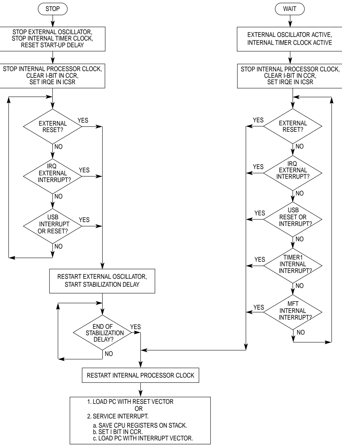
Figure 6-1. STOP and WAIT Flowchart
