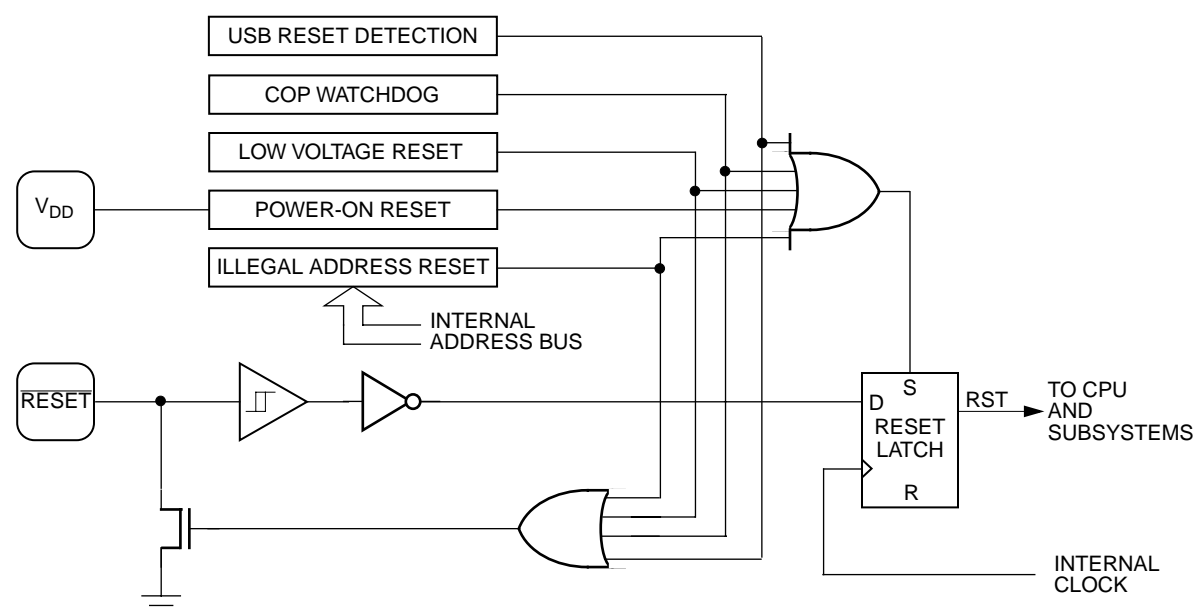
Figure 5-1. Reset Sources
