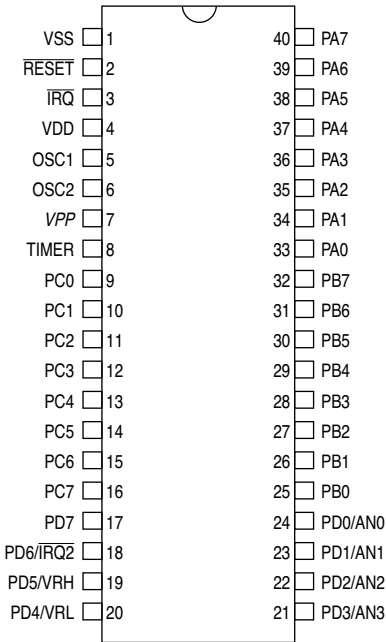
Figure 2-4 Pin Assignment for 40-pin PDIP
