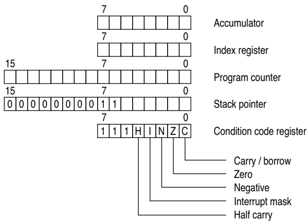
Figure 8-1 Programming model
