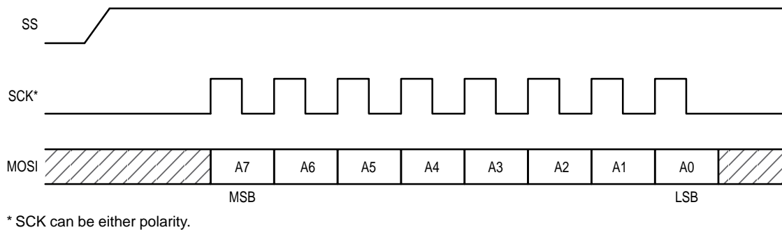
Figure 14. Address Byte Transfer Waveforms
