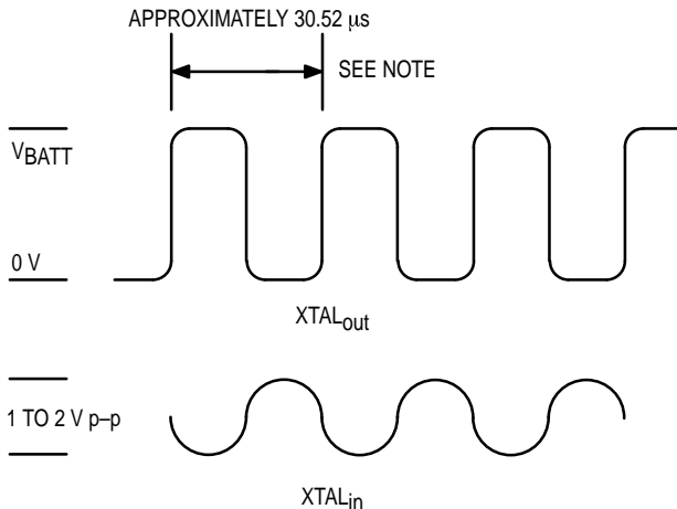
Figure 23. XTAL Waveforms
