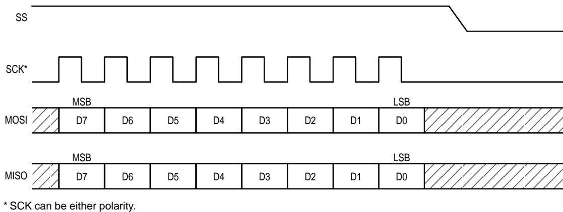
Figure 15. Read/Write Data Transfer Waveforms
