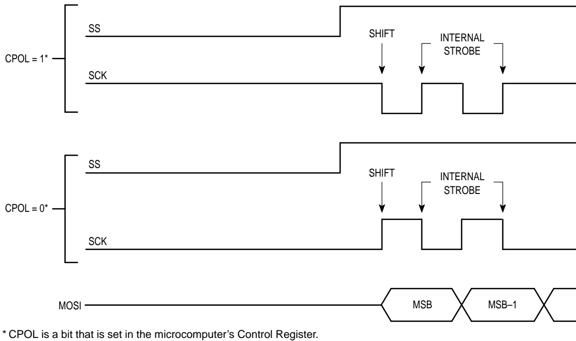
Figure 13. Serial Clock (SCK) as a Function of MCU Clock Polarity (CPOL)
