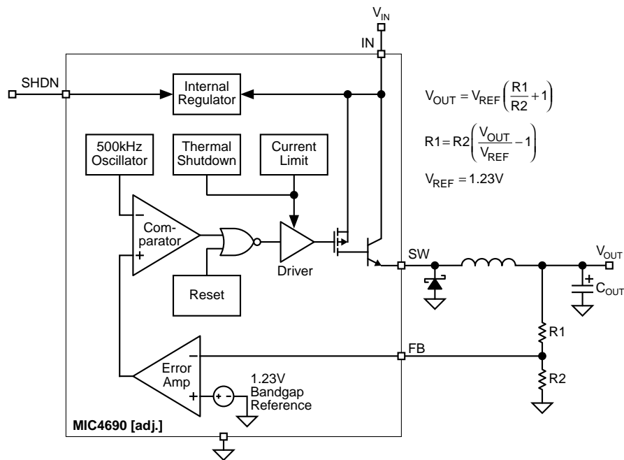
Adjustable Regulator
