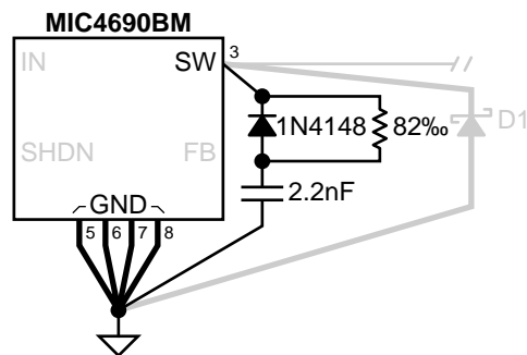
Snubber Circuit
