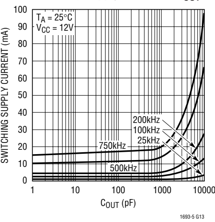
Switching Supply Current vs C OUT
