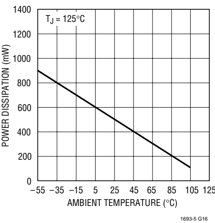
Thermal Derating Curve
