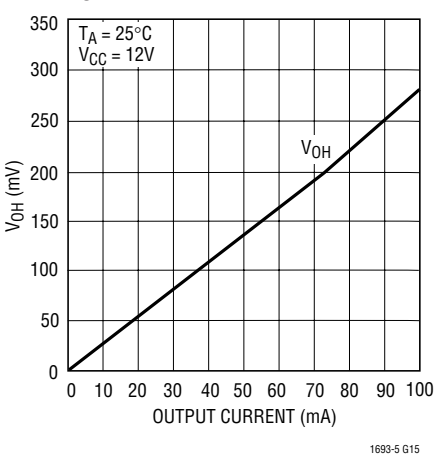
V OH vs Output Current
