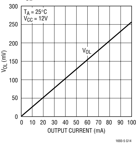
V OL vs Output Current
