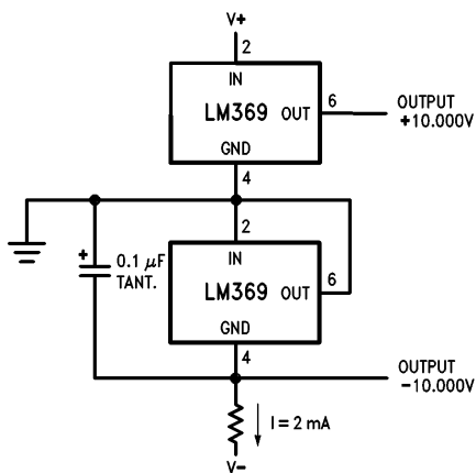
±10V Reference
