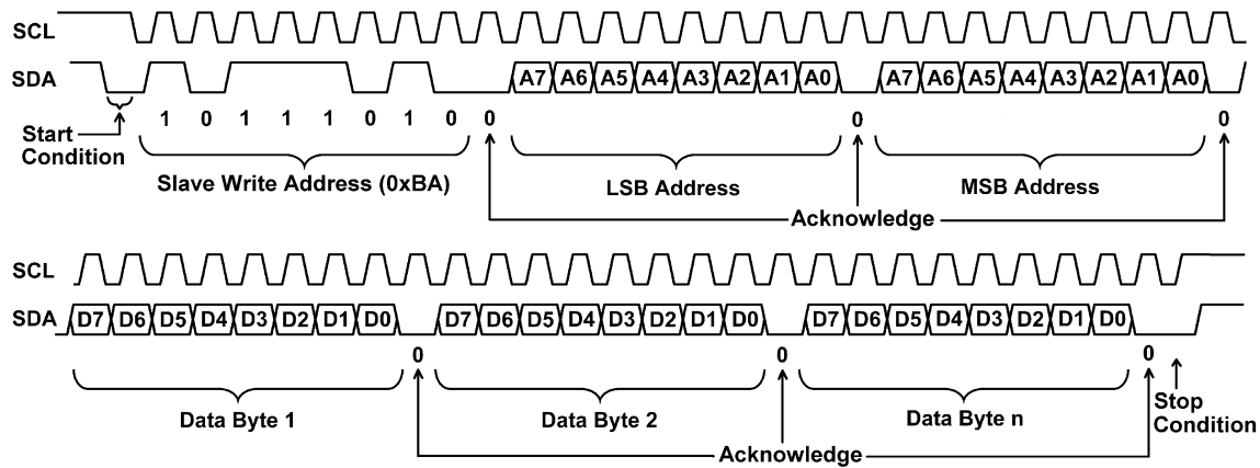
FIGURE 23. I²C Compatible Write Sequence
