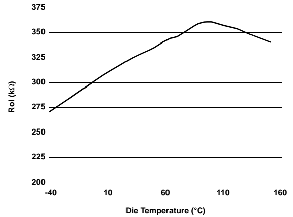
Transimpedance (RoI) vs Temperature
