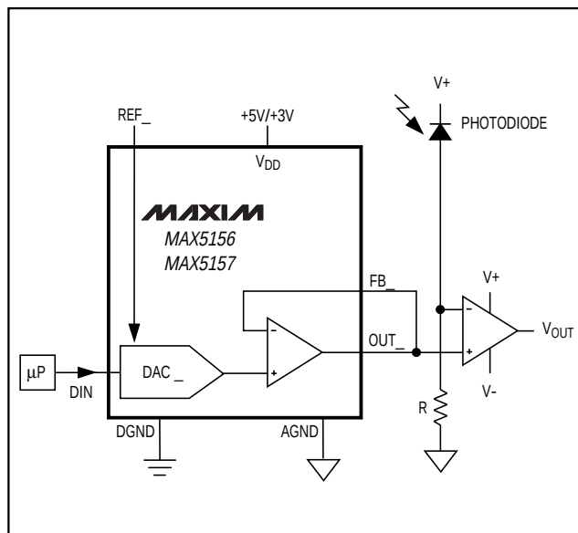
Figure 13. Digital Calibration
