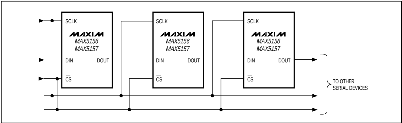
Figure 7. Daisy Chaining MAX5156/MAX5157s
