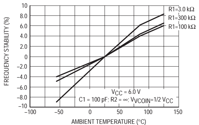
Figure 13C. Frequency Stability versus Ambient Temperature: V_{CC} = 6.0 V
