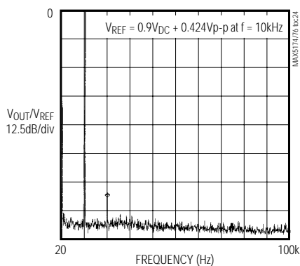
FFT PLOT
