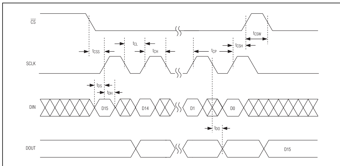
Figure 10. Timing Diagram
