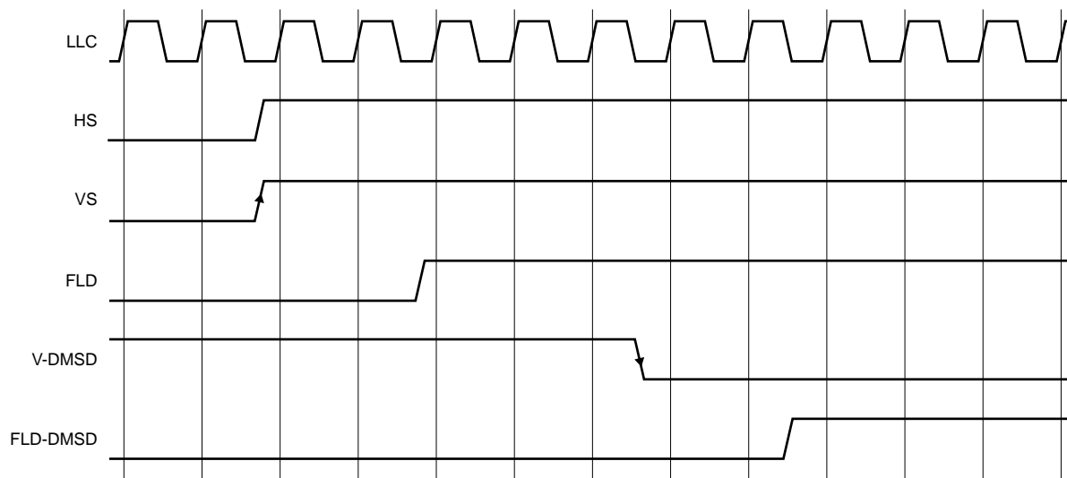
Fig.12 Timing of field detection EVEN-to-ODD for direct mode.
