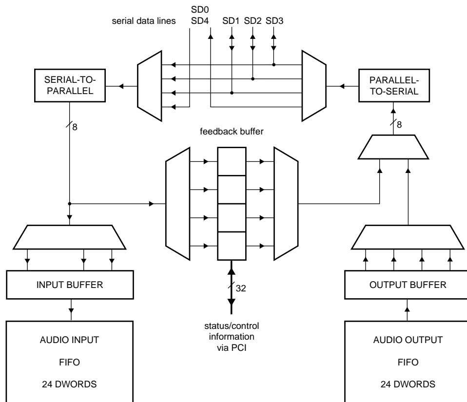
Fig.40 Audio data flow control in A1 and A2.
