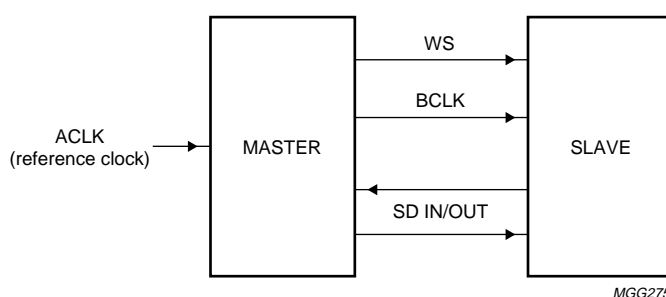
Fig.38 General application schematic of the audio interface.
