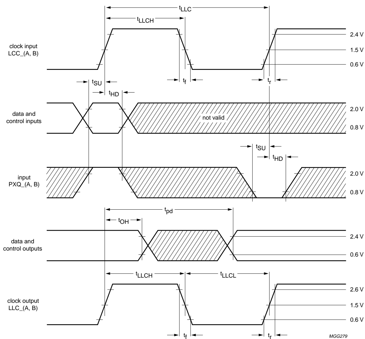
Fig.47 Clock/data timing.
