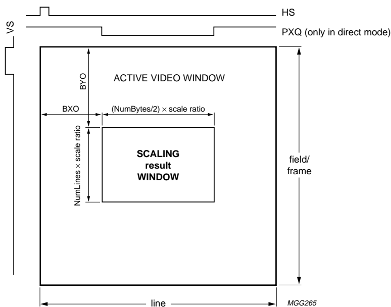
Fig.26 Reference signals for scaling window for direct and line memory mode.
