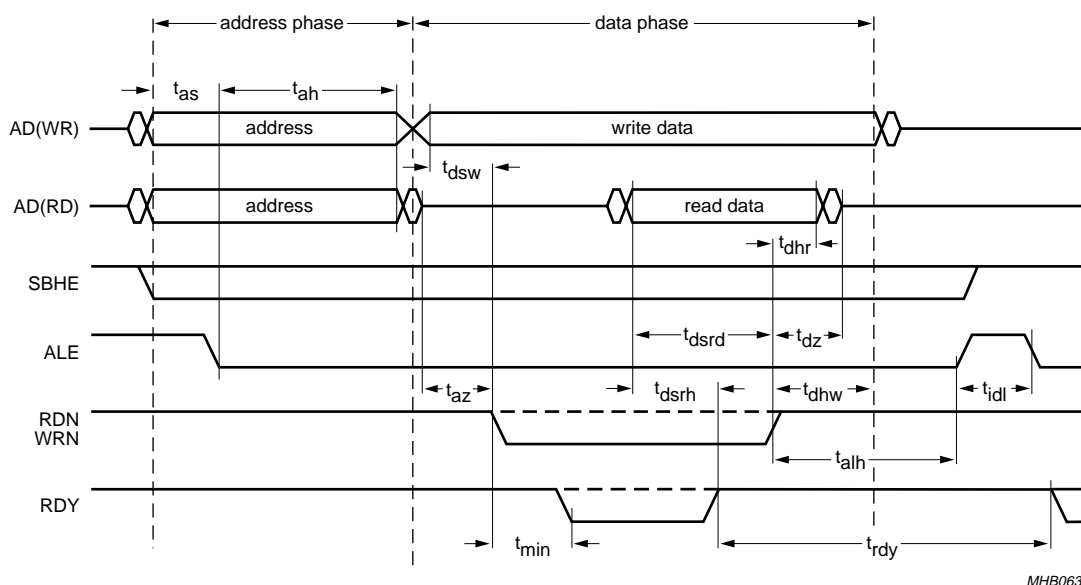
Fig.31 Intel style transfer.
