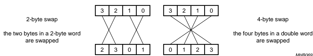
Fig.37 Endian swapping.
