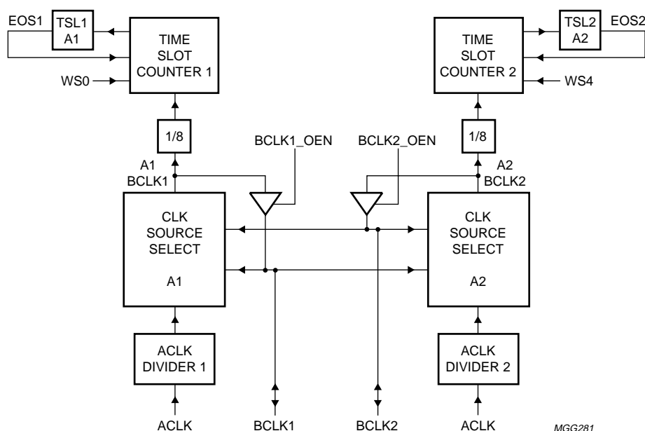
Fig.39 Audio clock control.
