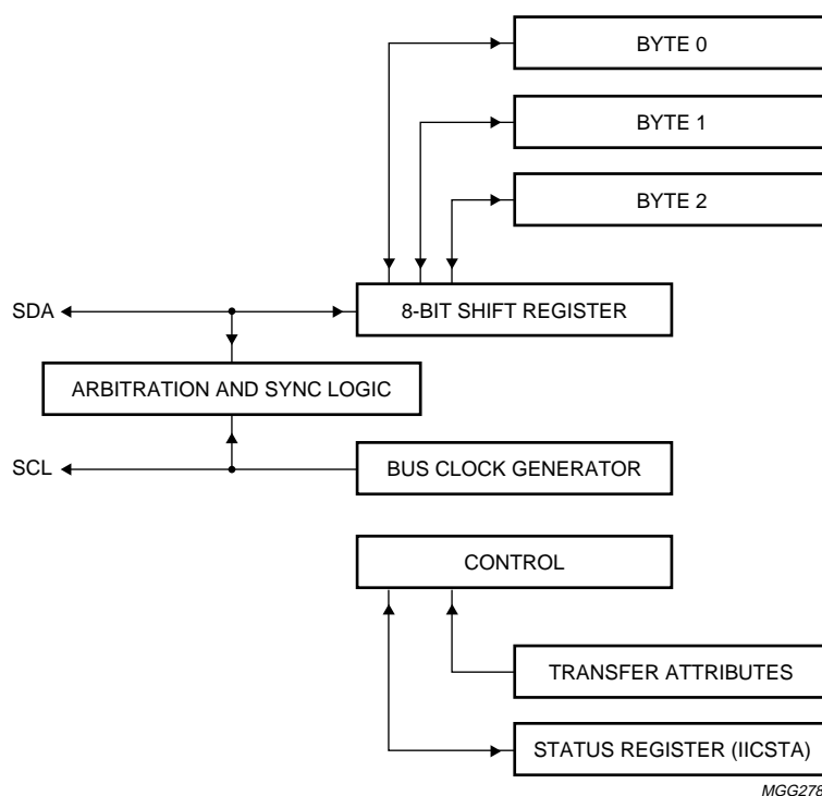
Fig.42 Block diagram of I 2 C-bus serial interface.
