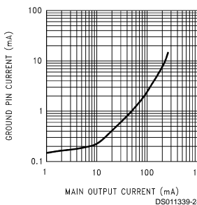
Ground Pin Current vs Main Load
