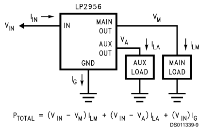
FIGURE 1. Current/Voltage Diagram
