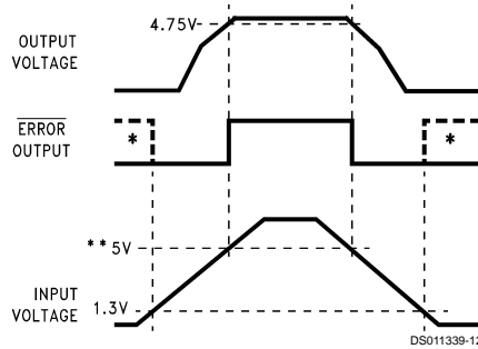
FIGURE 4. \overline{\text{ERROR}} Output Timing
