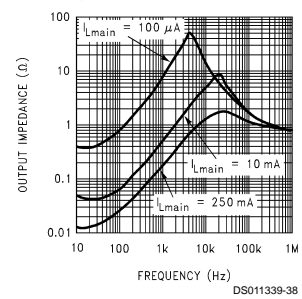
Output Impedance (Main Regulator)
