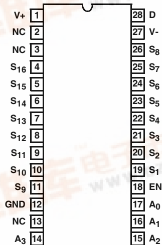
DG406/883 (CERDIP) TOP VIEW
