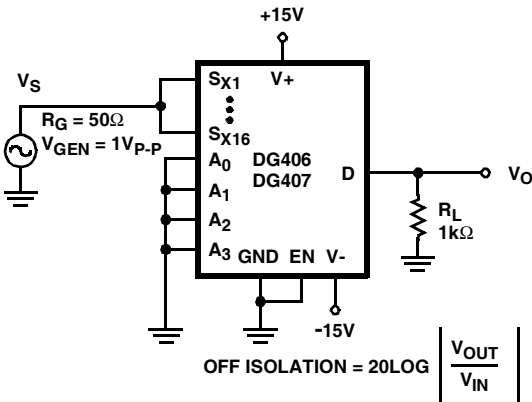
FIGURE 5. OFF ISOLATION
