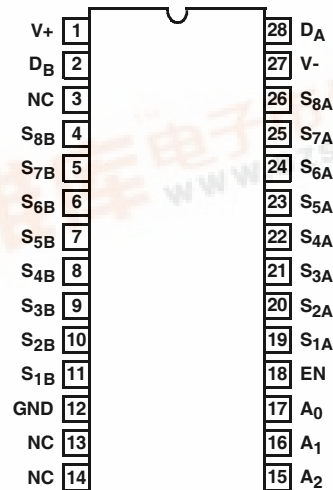
DG407/883 (CERDIP) TOP VIEW
