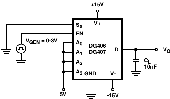
FIGURE 4. CHARGE INJECTION
