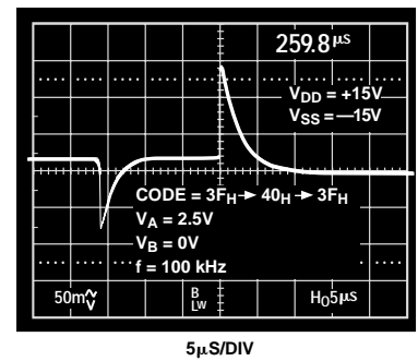
Figure 16. Midscale Transition Glitch
