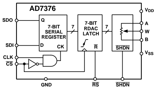
Figure 41. Block Diagram
