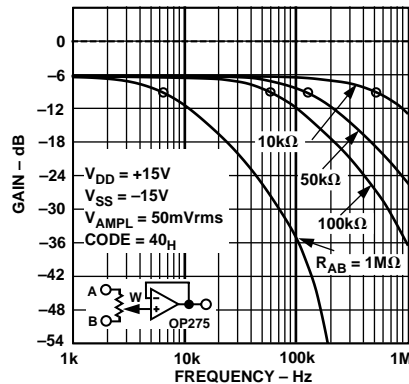
Figure 21. -3 dB Bandwidth vs. Nominal Resistance
