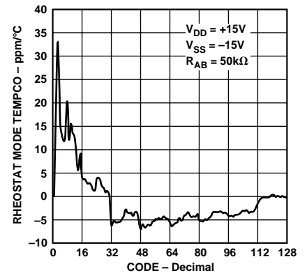
Figure 13. \Delta R_{WB}/\Delta T Rheostat Mode Tempco
