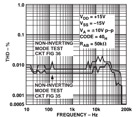
Figure 19. Total Harmonic Distortion Plus Noise vs. Frequency
