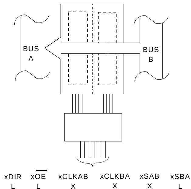
REAL-TIME TRANSFER BUS B TO A
