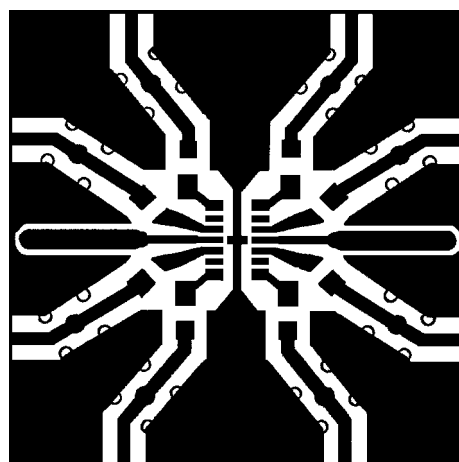
Figure 20. Component Side
