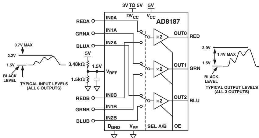
Figure 10. DC-Coupled (Bypassing and Logic Not Shown)
