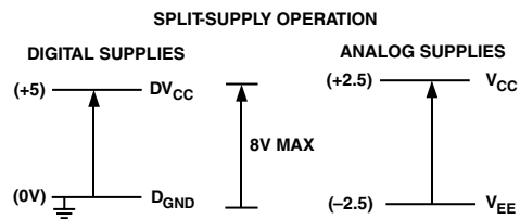
Figure 9. Split-Supply Operation
