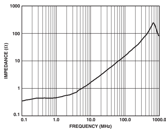
TPC 23. AD8187 Enabled Output Impedance vs. Frequency
