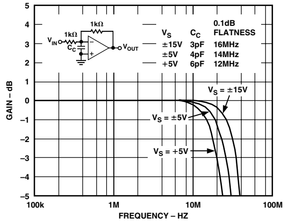
Figure 22. Closed-Loop Gain vs. Frequency, Gain = -1
