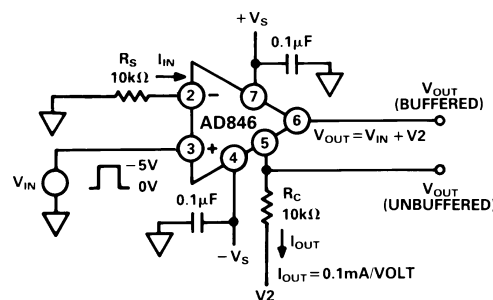
Figure 48. AD846 Connected as a Level Shift Amplifier
