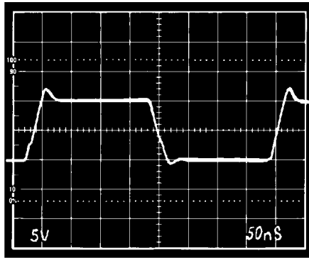
Figure 27b. Large Signal Pulse Response, Gain of 10
