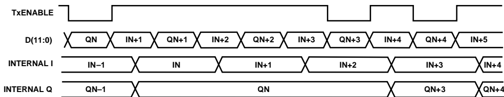
Figure 27. Continuous Mode Input Timing—TxENABLE Static High
