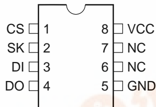
8-Pin PDIP
