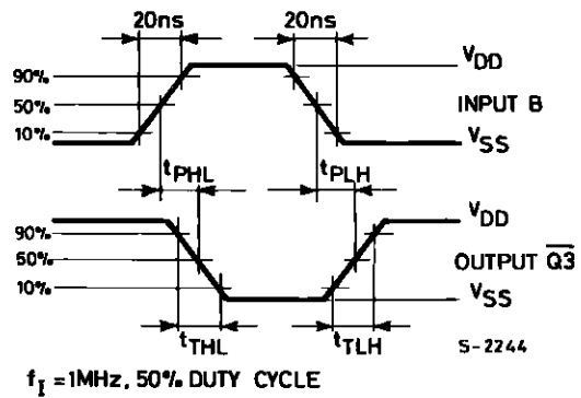
HCC/HCF4556B Input to \overline{Q3} Output Dynamic Signal Waveforms
