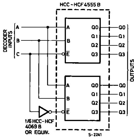
1 of 8 Decoder using HCC/HCF 4555B
